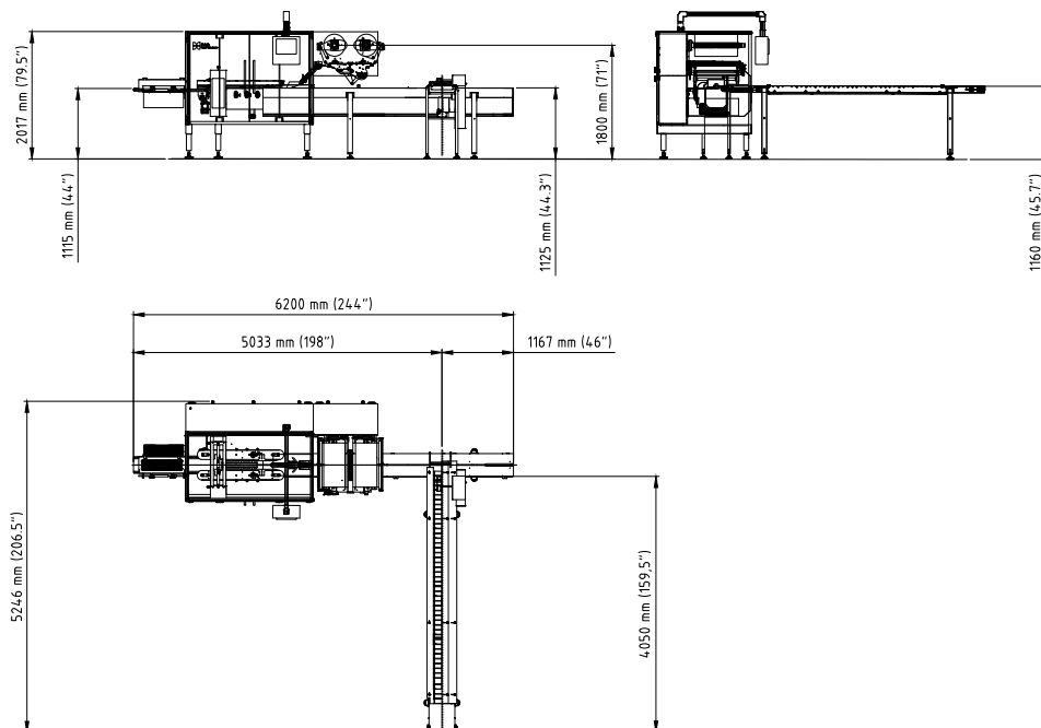
Sealing Station
